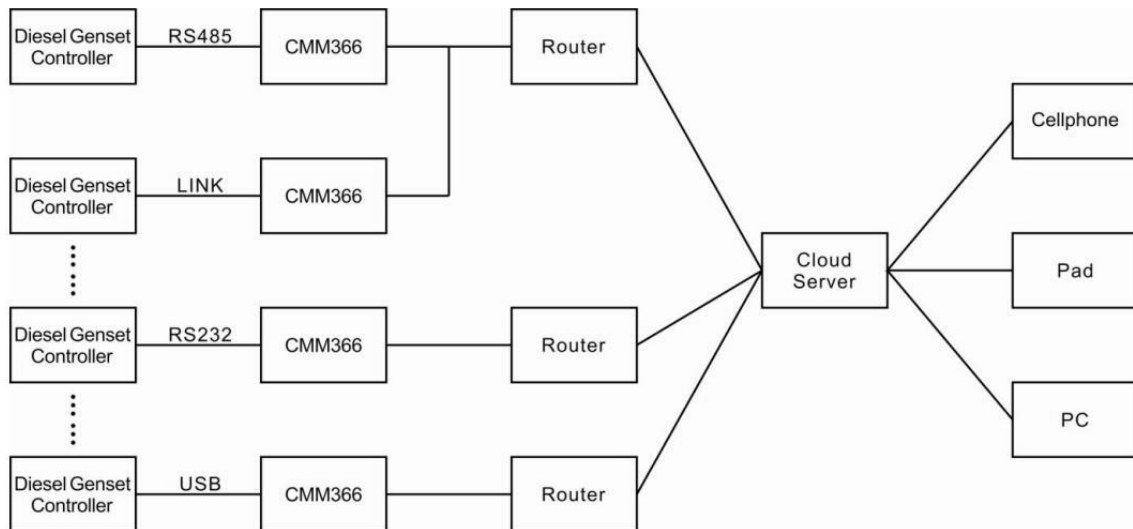
图1 CMM366-3G System Diagram
